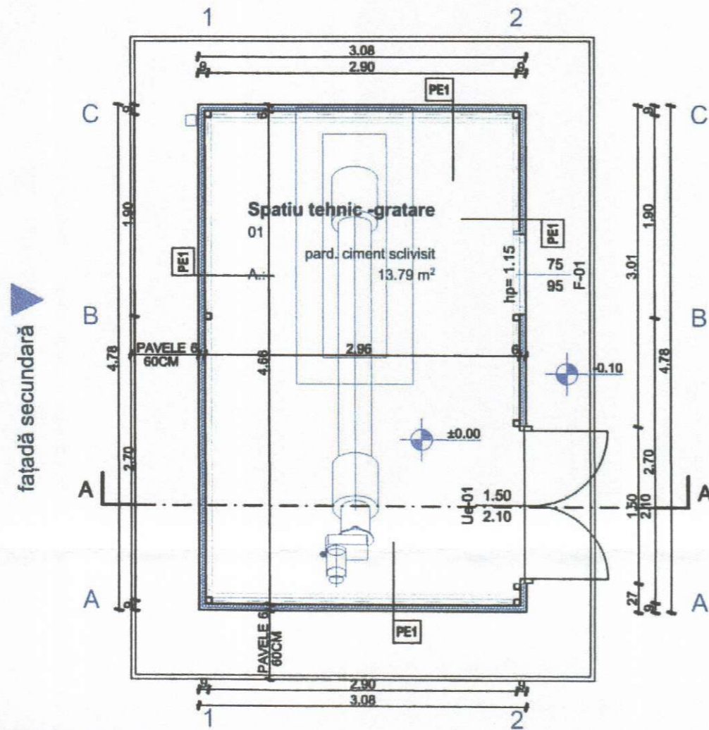
PLAN COTA +0.00, SC.1:50
